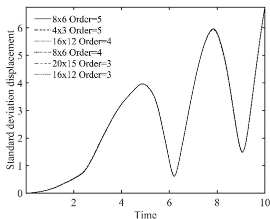
Fig. 9 Standard deviation vertical displacement history of Cook's membrane under triangular dynamic loading at node A
