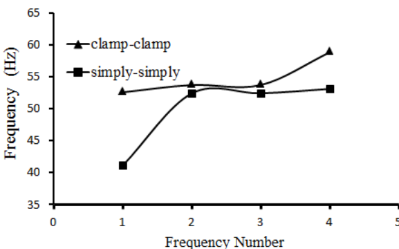
Fig. 11 comparison the Variation of the natural frequencies for the simply-simply FML cylindrical shell with AL/GE-1-5&[90/0/0/90] construction
