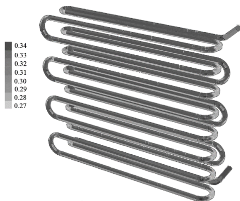
Fig. 6 The velocity gradient (m/s) in simulation system
