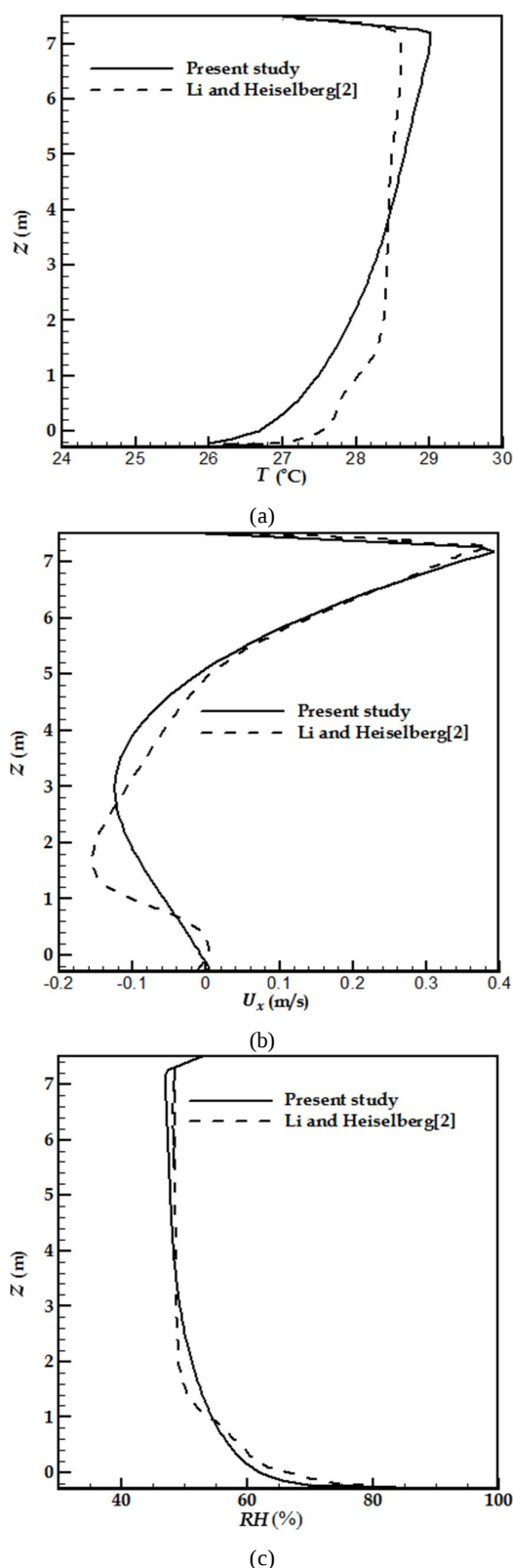
Fig. 6 Present study results compared with results of Li and Heiselberg[2] (a) Temperature (°C), (b) Velocity in x direction (m/s), (c) Relative humidity (%)
