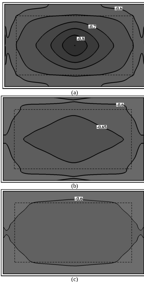
Fig. 12 Thermal comfort field at the height of (a) 0.1 m (b) 1.1 m (c) 1.8 m
