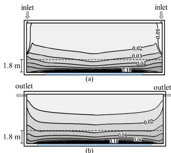
Fig. 10 Concentration field of chlorine in \text{mg/m}^3 at (a) plane A (b) plane B
