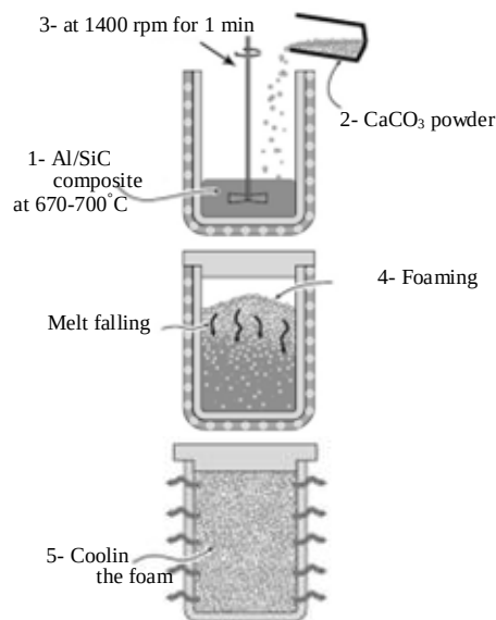
Fig. 2 The stages of foam production
