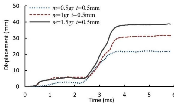
Fig. 9 Diagram of the deflection of the circular copper plate's center with 0.5 mm thickness under the loading of explosive charges with different weights
