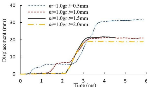
Fig. 15 Diagram of deflection of circular copper plate's center with different thicknesses under the 1 gram T.N.T loading
