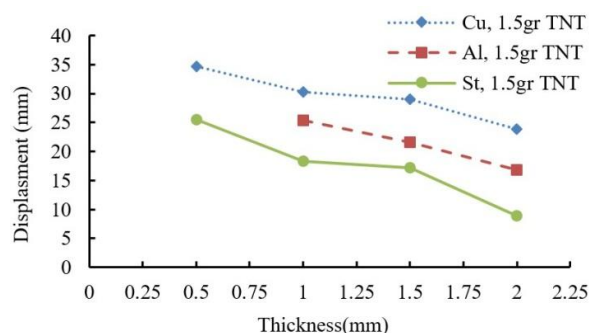
Fig. 23 The maximum experimental deflection of the center of plate under the loading of 1.5 gram explosive charge for different thicknesses and materials
