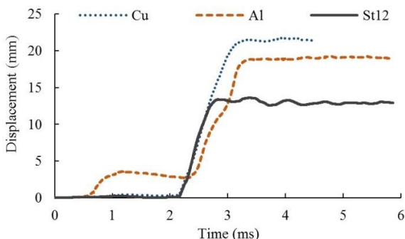
Fig. 16 Diagram of deflection of circular plate's center with different materials and the 1.5 millimeter thickness under the 1 gram T.N.T loading
