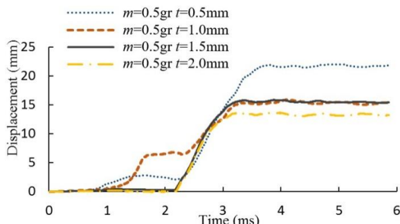
Fig. 14 Diagram of deflection of circular copper plate's center with different thicknesses under the 0.5 gram T.N.T loading
