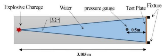
Fig. 2 Schematic view of the explosive shock tube
