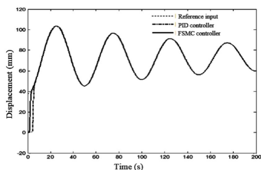
Fig.14 Response of closed loop system to input with frequency 0.02 Hz
