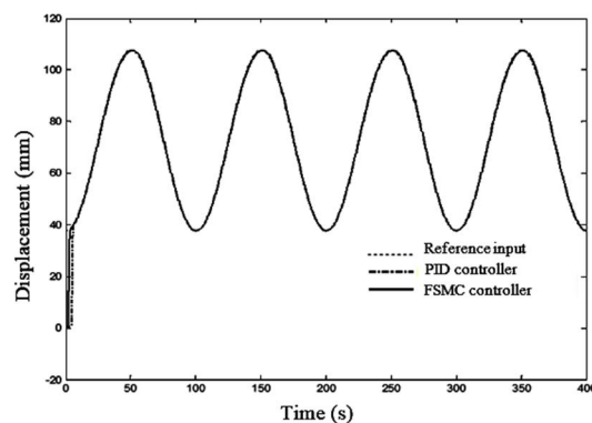
Fig.13 Response of closed loop system to input with frequency 0.01 Hz
