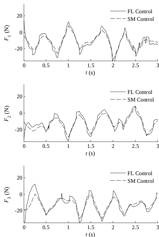
Fig. 8 Control signals
