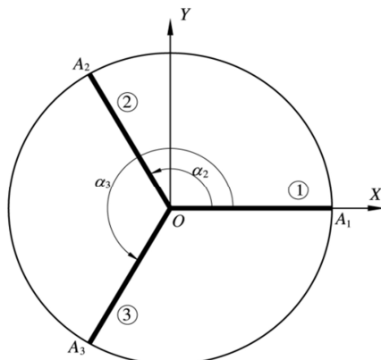
Fig. 3 Upper view of a 3[P2(US)] robot
