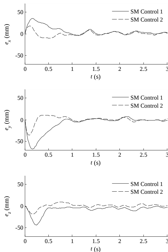
Fig. 12 Error components
