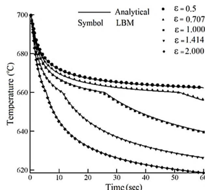
Fig. 8 Temperature variation for a point located 1 mm long aside the left wall
