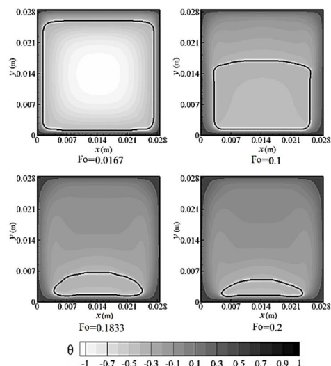
Fig. 16 Dimensionless temperature field and position of melting front for the case of free solid phase melting related to \gamma = 1
