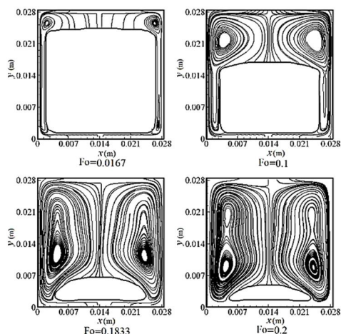
Fig. 17 Streamlines around the free solid phase during melting, \gamma = 1
