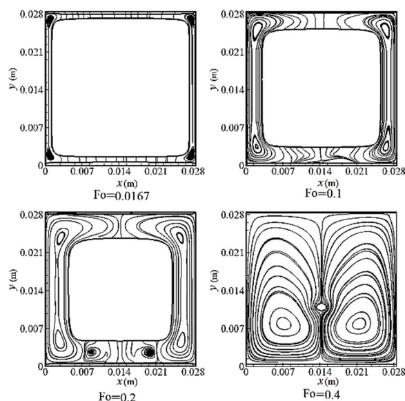
Fig. 15 Streamlines around the fixed solid phase during melting, \gamma = 1
