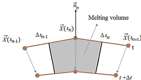
Fig. 4 Energy conversion on the finite control volume
