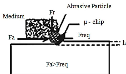
Fig. 1 Machining forces in the AFM [2]
