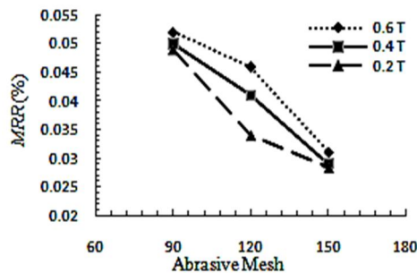
Fig. 5 The effect of size of abrasive particles on the material removal rate in different field intensity (workpiece hardness: 35 HRC)
