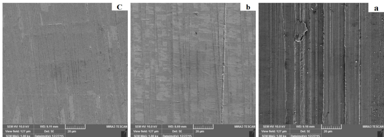
Fig. 16 a) SEM image of the surface before MAFM process in 1000X b) SEM image of workpiece surface with 35 HRC after MAFM in 1000X (mesh=150, H=0.6) c) SEM image of workpiece surface with 55 HRC after MAFM in 1000X (mesh=150, H=0.6)
