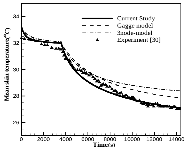
Fig. 7 Comparison of measured mean skin temperature from one female subject [30] and simulated mean skin temperature by Gagge model, 3node-model and current study.
