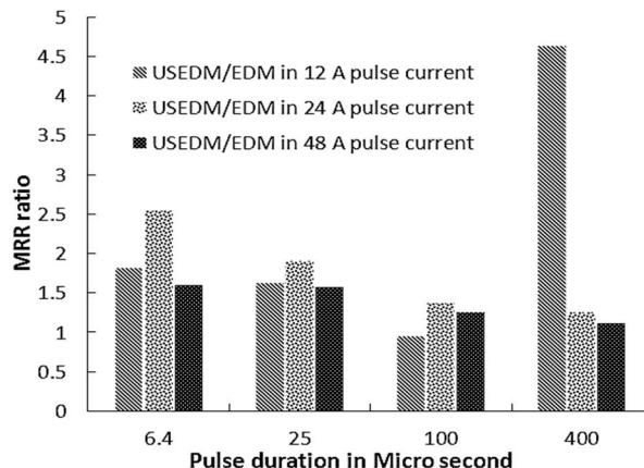
Fig. 3 MRR ratio versus pulse duration in different pulse current.
