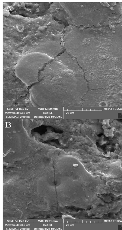
Fig. 6 SEM micrograph of produced surfaces in processes A) EDM, B) USED, in 24 A pulse current and 100 \mu s pulse duration
