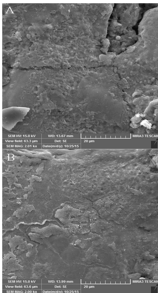
Fig. 5 SEM micrograph of produced surfaces in processes A) EDM, B) USED, in 12 A pulse current and 100 μs pulse duration
