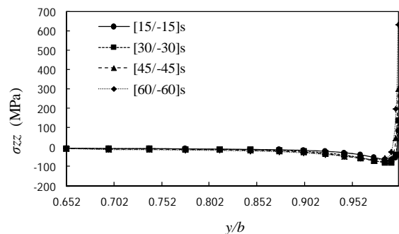
Fig. 12 Transverse normal stress \sigma_{zz} versus y/b non dimensional coordinate in the angle-ply laminate at the \theta - \theta interface under extension loading.
