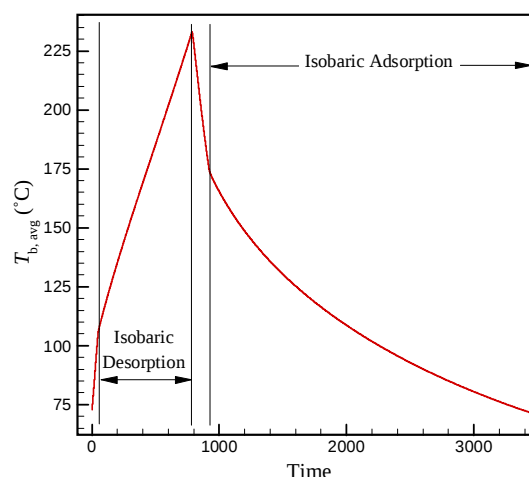
Fig. 7 Time variation of the averaged adsorber bed temperature in exhaust driven adsorption cooling system
