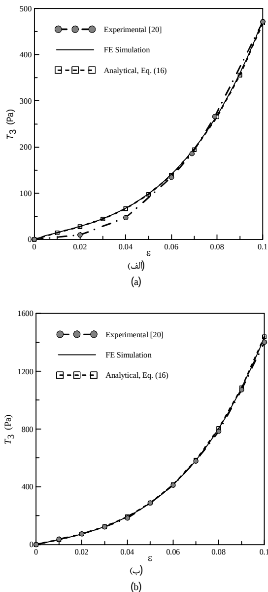
Fig. 5 Experimental, analytical and numerical stress-strain curves (hyper-viscoelastic), (a) \dot{\epsilon}=0.0011\text{s}^{-1} , (b) \dot{\epsilon}=0.4167\text{s}^{-1}
