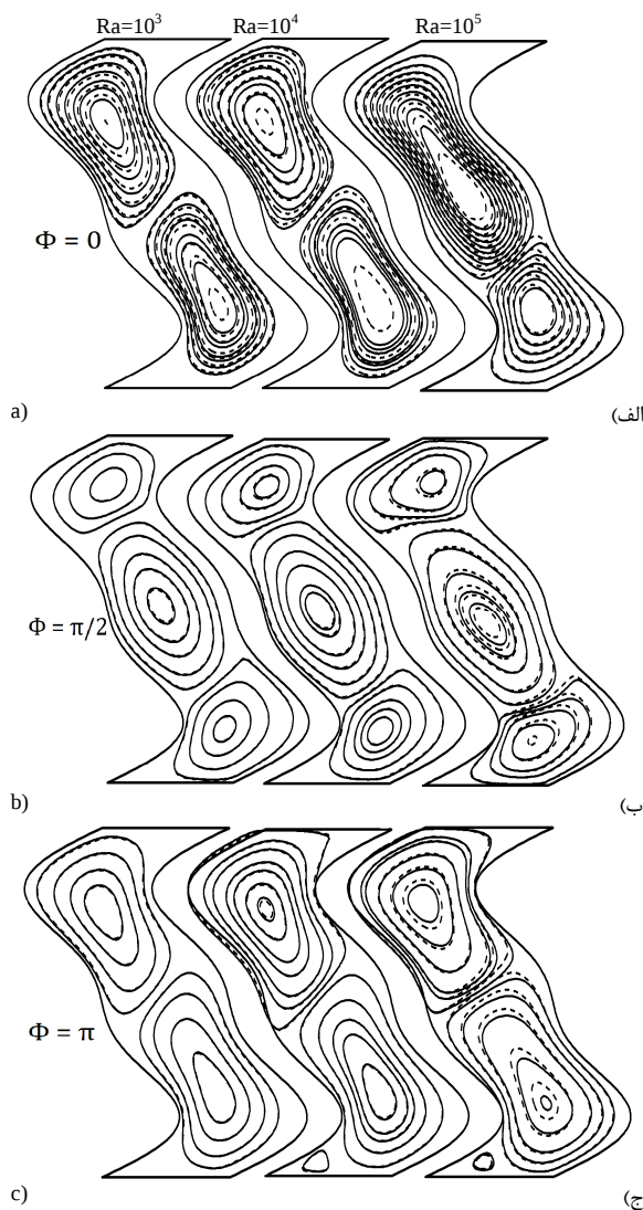
Fig. 13 Streamlines contours for nanofluid (dashed line) and pure fluid (solid line) for different Rayleigh numbers and phase deviations. ( \alpha_1=0.5 , R_a=1/2.5 , \lambda=2 , \phi=0.04 )
