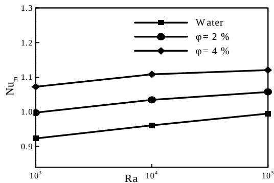
Fig. 12 Variation of mean Nusselt number with Rayleigh number for different nanoparticle volume fractions. ( \alpha_1=0.5 , R_a=1/2.5 , \lambda=2 , \Phi=0 )
