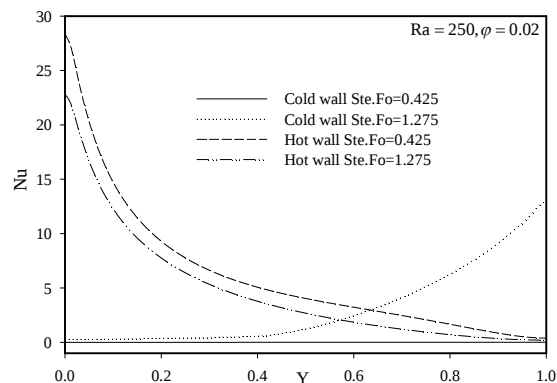
Fig. 9 Local Nusselt number along hot and cold walls of the cavity for different times ( Ra = 250, \phi = 0.02, \varepsilon = 0.3 )
