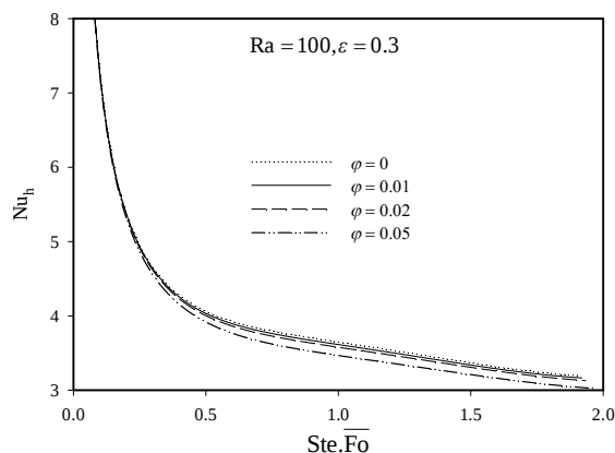
Fig. 12 Variation of the hot wall average Nusselt number with time (Ste.Fo) for different \phi ( Ra = 100, \varepsilon = 0.3 )
