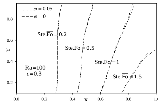
Fig. 11 Melting line advance in cavity over time (Ste.Fo = 0.2, 0.5, 1, 1.5) for ( Ra = 100, \varepsilon = 0.3, \phi = 0, 0.05 )
