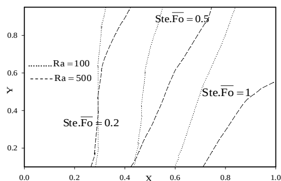
Fig. 10 Melting line advance and shape in cavity over time (Ste.Fo = 0.2, 0.5, 1) for ( Ra = 100, 500, \phi = 0.02, \varepsilon = 0.3 )
