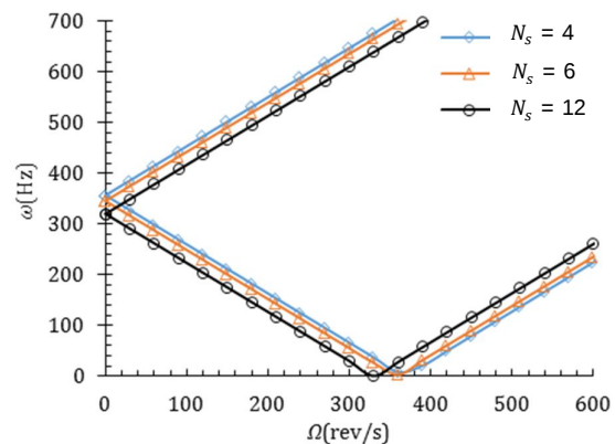
Fig. 10 The effect of stiffener numbers on natural frequency for n=1
