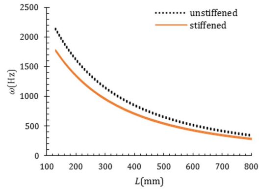
Fig. 18 Comparison The effect of length on frequency of stiffened and unstiffened cylindrical shell for n=1
