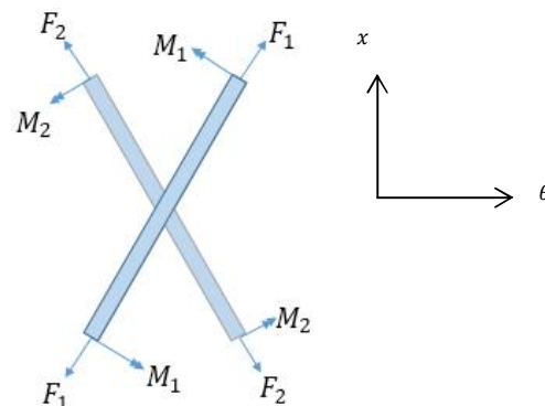
Fig. 2 Free body diagram of forces and moments for a unit cell
