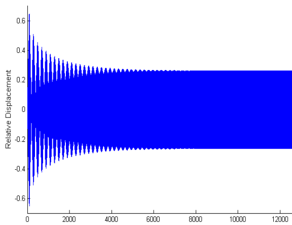
Fig. 9 The time history diagram of the system for d=0.5 , F=1 , \sigma=-6 and \alpha=0.2
