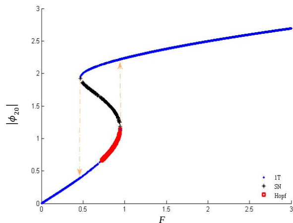
Fig. 14 The Force-response diagram of the system for d=0.24 , \sigma=1 and \alpha=0.2
