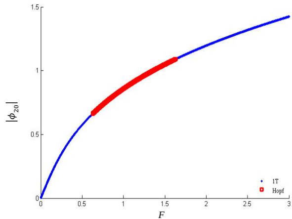
Fig. 13 The Force-response diagram of the system for d=0.5 , \sigma=1 and \alpha=0.2
