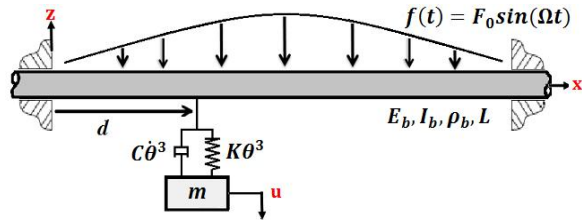
Fig. 1 A schematic view of horizontal clamped-clamped beam with nonlinear energy sink under harmonic external load
