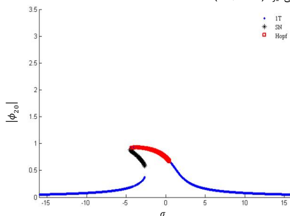
Fig. 7 The Frequency-response diagram of the system for d=0.5 , F=0.5 and \alpha=0.2 (point 1 in Fig. 4)
