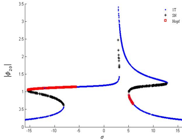
Fig. 10 The Frequency-response diagram of the system for d=0.5 , F=2 and \alpha=0.2 (point 3 in Fig. 4Fig.)
