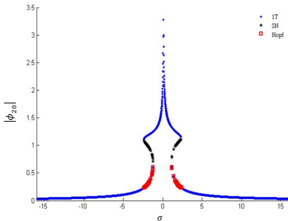
Fig. 11 The Frequency-response diagram of the system for d=0.12 , F=2 and \alpha=0.2 (point 10 in Fig. 6)
