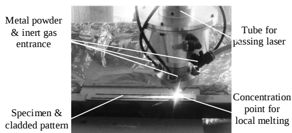
Fig. 1 Cladding of stainless steel with CO 2 laser
