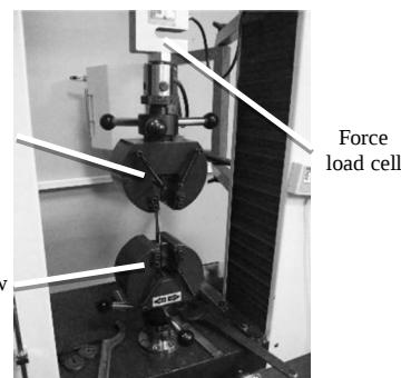
Fig. 4 Extracting joint strength of hybrid via uniaxial test
