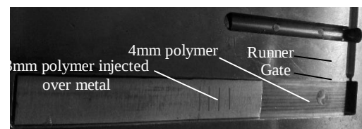
Fig.7 metal position in cavity for tension test specimens
