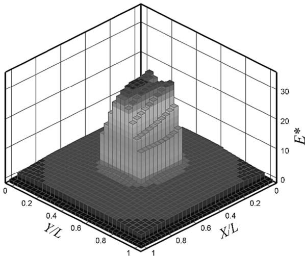
Fig. 9 Dimensionless emissive power distribution over the entire enclosure medium, \varepsilon = 0.5 and \tau = 1 , with diffuse-nongray design surface
