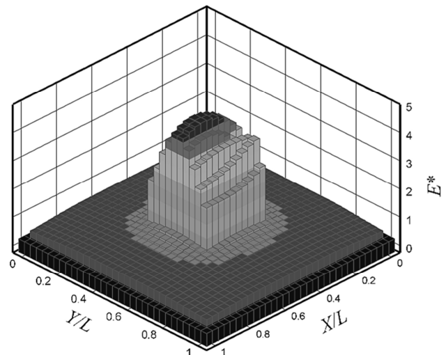
Fig. 16 Dimensionless emissive power distribution over the entire enclosure medium, \varepsilon = 0.5 and \tau = 1 , with diffuse-gray design surface, \varepsilon_{dg} = 0.5
