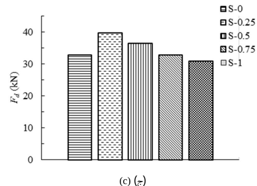
Fig. 8 Mean dynamic force: (a) hexagonal, (b) octagonal, (c) square
