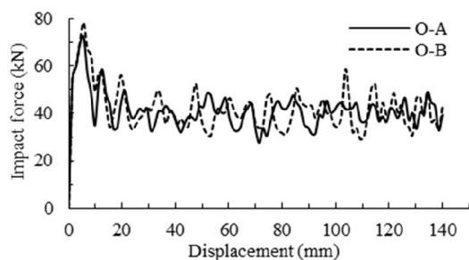
Fig. 15 Force-displacement curve for octagonal double walled tubes
