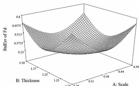
Fig. 10 Standard error of tubes for selected design space
