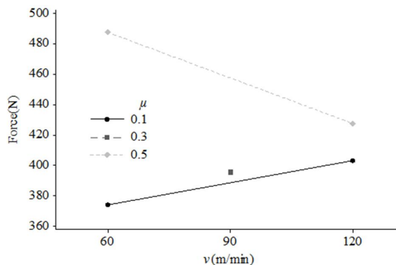
Fig. 5 Interaction plot of friction and federate on force on the tool
