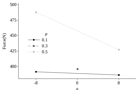
Fig. 6 Interaction plot of friction coefficient-rake angle on force on the tool
