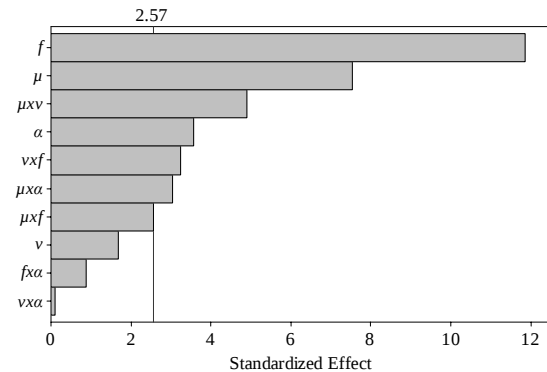
Fig. 4 Pareto chart of force on the tool
