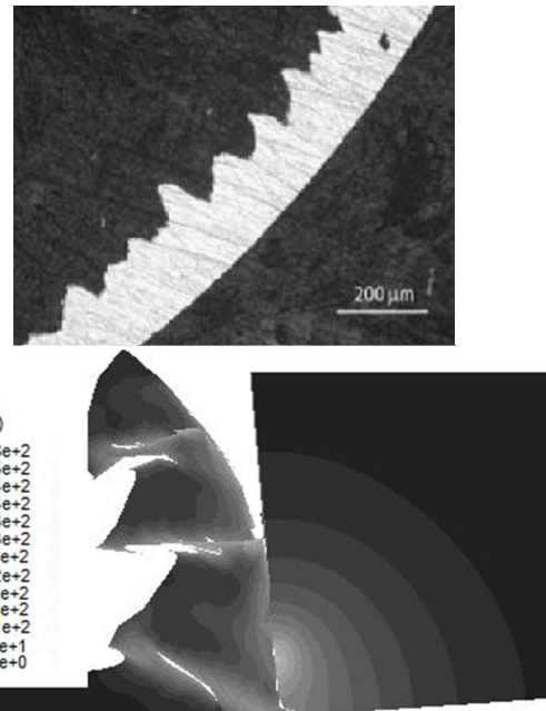
Fig. 2 Sawtooth chip formation in simulated and experimental
