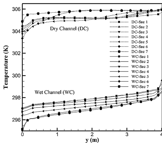
Fig. 6 Temperature distribution on vertical sections. Comparison of dry and wet channels
