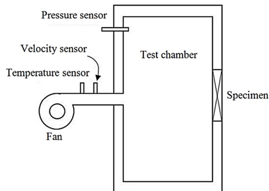
Fig. 2 Schematic of tester device
