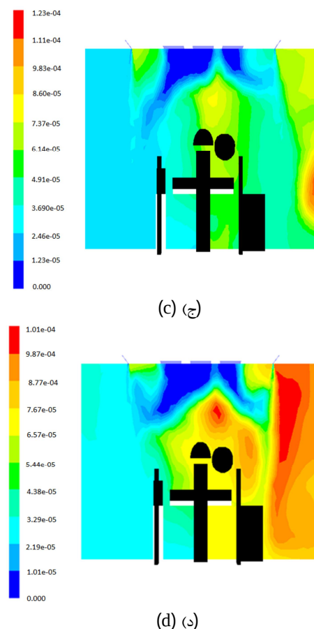
Fig. 3 Contours of mass fraction of contaminant for air velocity (a) 0 m/s (b) 2.37 m/s (c) 3.37 m/s (d) 4.37 m/s
