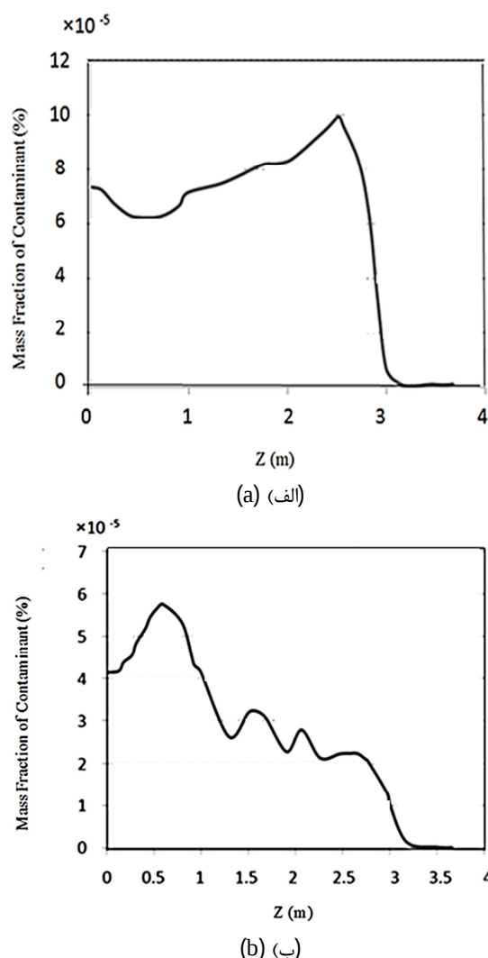
Fig. 4 Variation of contamination respect to the height of operating room for air velocity (a) 0 m/s (b) 2.37 m/s
