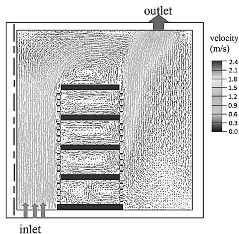
Fig. 5 velocity vectors for v_{in} = 0.8 (m/s)
