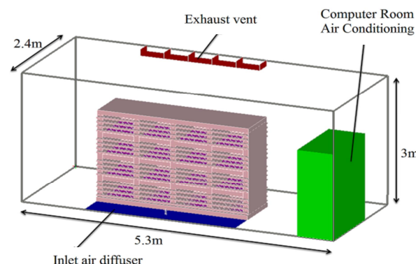
Fig. 3 Configuration of the space model
