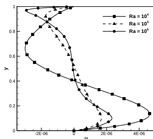
Fig. 3 U-velocity along vertical centerline
