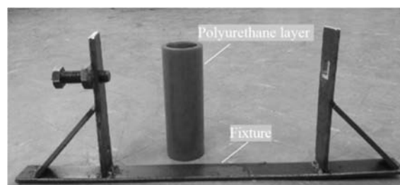
Fig. 8 Manufactured fixture
