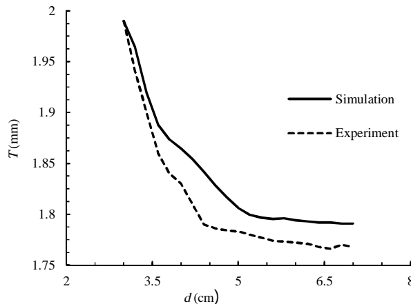
Fig. 13 Thickness of bulged sample along path (a1)
