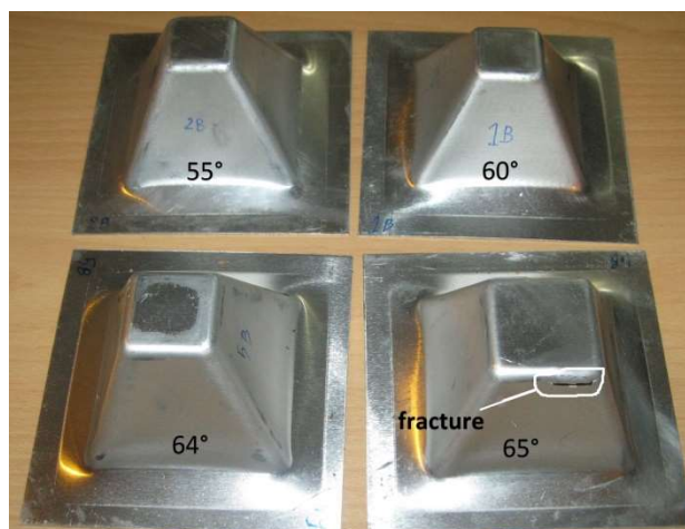
Fig. 16 Formed parts for determination of maximum formable angle at 1000 RPM tool rotation speed
