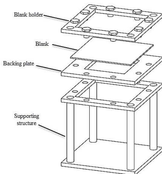
Fig. 8 Sheet clamping mechanism for single point incremental forming
