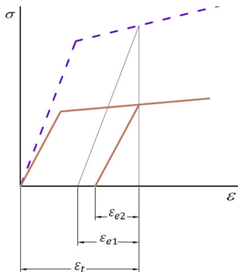
Fig. 2 Schematic representation of the dependence of elastic strain to yield stress
