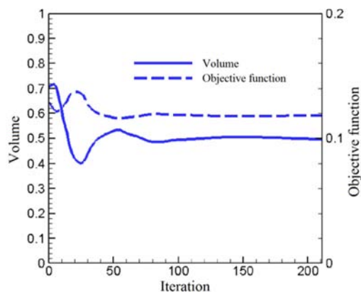
Fig. 6 Iteration histories of the objective function and volume constraint
