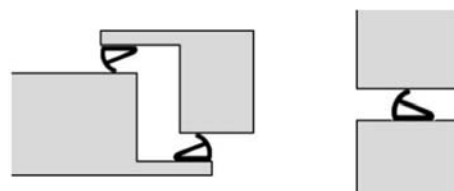
Fig. 5 Gasket placement into gap
