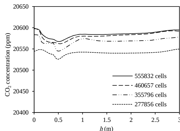
Fig. 7 CO_2 concentration on the line (x = 1.5, x = 1.5) in terms of height شکل 7 غلظت CO_2 روی خط (x = 1.5, z = 1.5) برحسب ارتفاع
