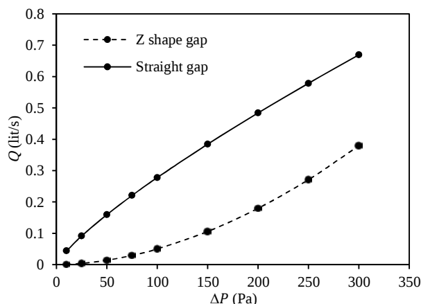
Fig. 15 The average results of air infiltration rate for straight and Z shape gap
