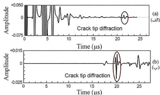
Fig. 12 (a) The crack tip diffracted echo received by the transducer A, (b) The crack tip diffracted echo received by the transducer B
