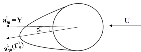
Fig 4 Initial orientation of U shaped cable under wind flow
