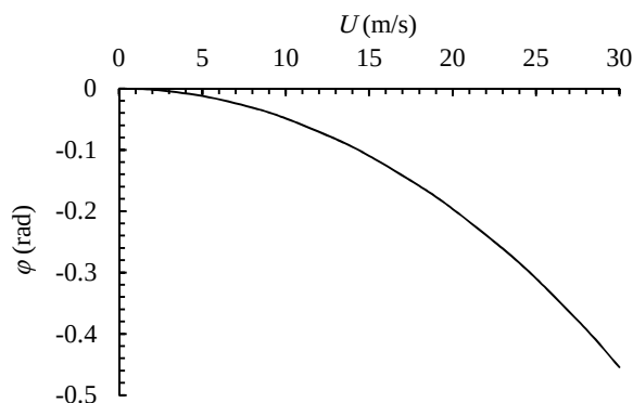
Fig. 8 Nonlinear equilibrium path
