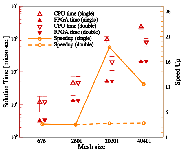
Fig. 10 Time duration and speedup for Laplace solution
