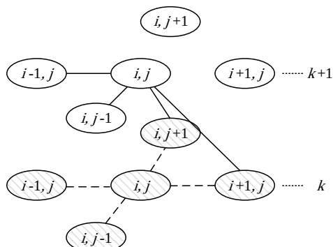
Fig. 6 Stencil of the point Gauss-Seidel method
