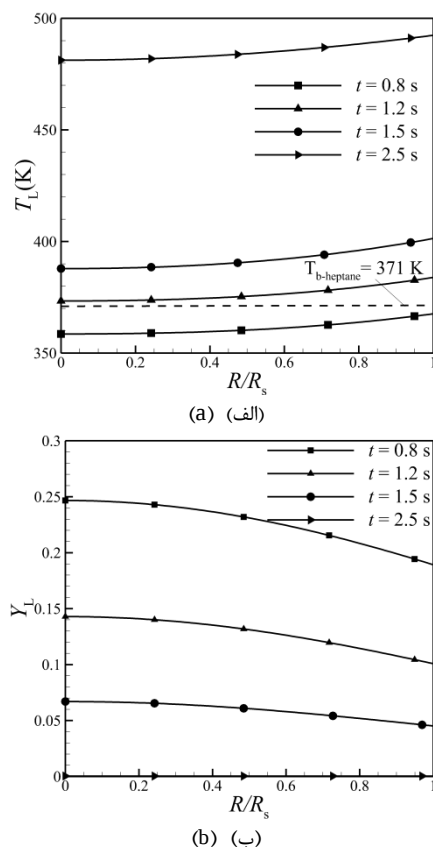
Fig. 11 Internal liquid distribution a) Temperature b) mass fraction
