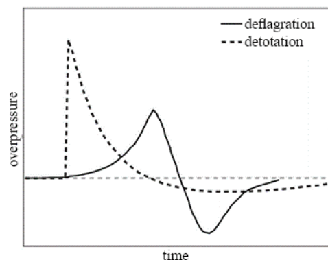
Fig.1 two mechanism for explosion [4]
