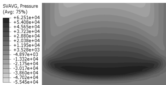
Fig.8 incident blast wave (Pa)
