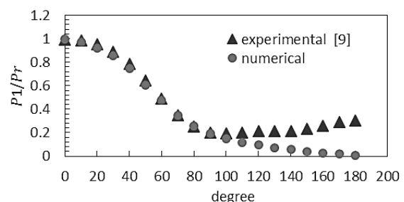
Fig.15 comparison of current numerical result with experimental result in [9]
