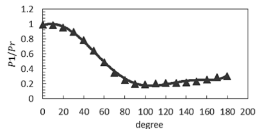
Fig.6 the suggested curve by Yasserli for P_1/P_r from zero to 180 degree [9]
