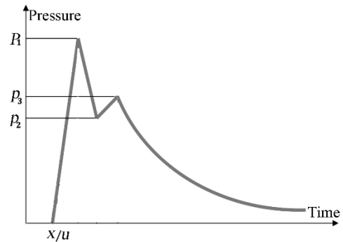
Fig.5 the pressure-time curve presented in [9]
