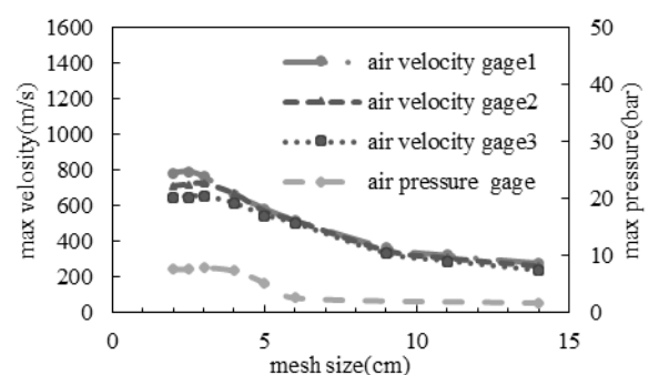
Fig.11 mesh convergence study
