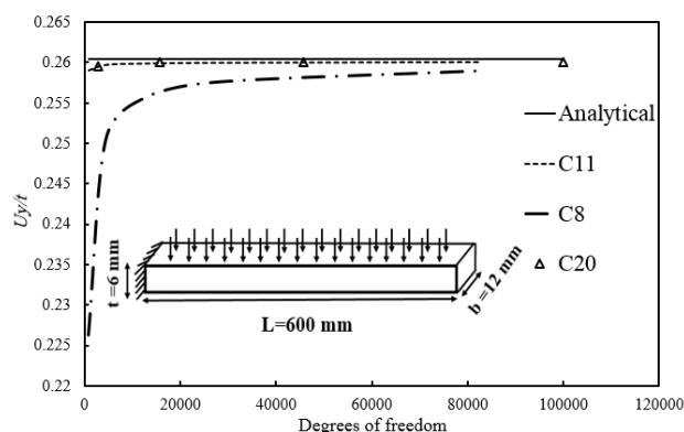
Fig. 6 Dimensionless lateral displacement of beam due to degrees of freedom for C8, C11 and C20 elements
