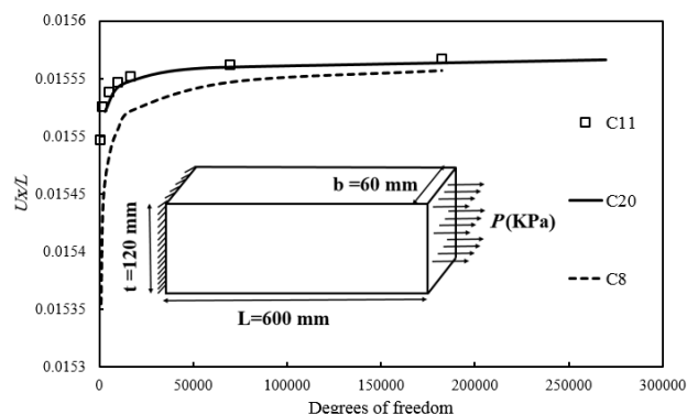
Fig. 13 Dimensionless in-plane displacement at the beam tip due to degrees of freedom for C8, C11 and C20 elements
