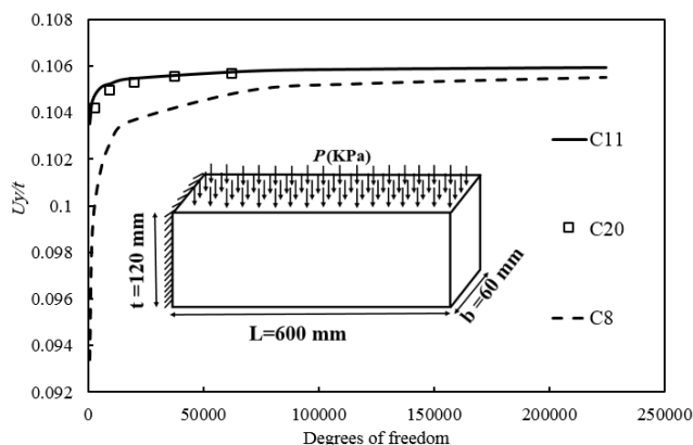
Fig. 14 Dimensionless lateral displacement in Y direction due to degrees of freedom for C8, C11 and C20 elements
