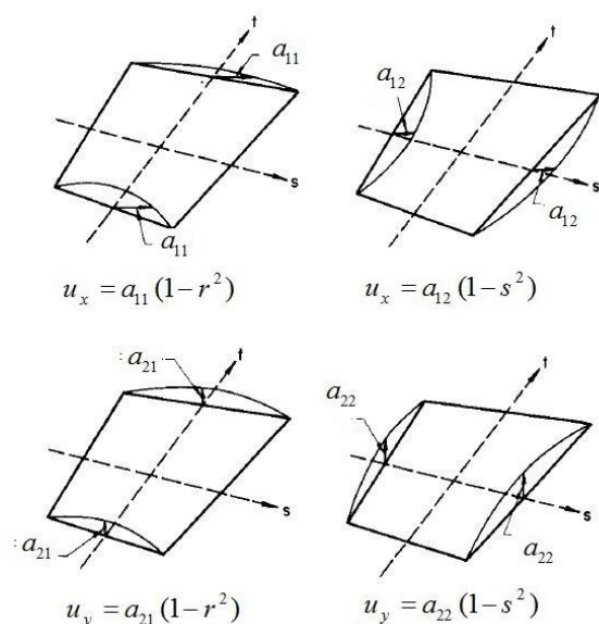
Fig.2 Incompatible displacement mode for quadrilateral element [3]
