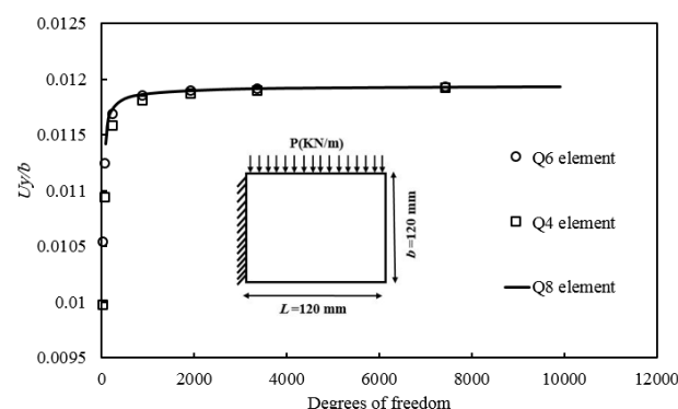
Fig.10 Dimensionless displacement in loading direction due to degrees of freedom for Q4, Q6 and Q8 elements
