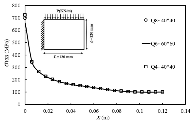
Fig. 11 Von-Mises stress through the plate length for Q4, Q6 and Q8 elements at y=120\text{mm} and 0 < x < 120\text{ mm}
