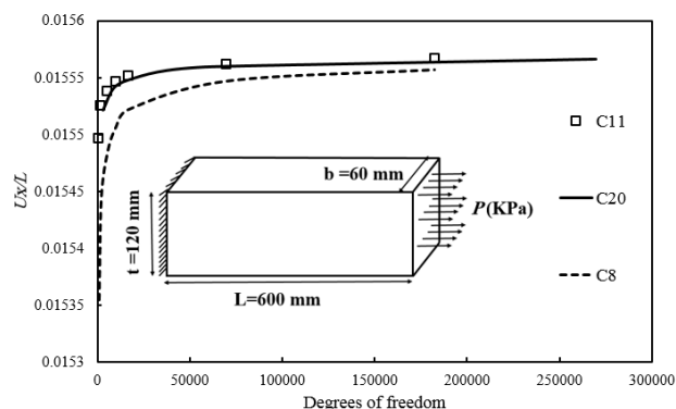
Fig. 15 Von-Mises stress behavior for C8, C11 and C20 elements with various Degrees of freedom
