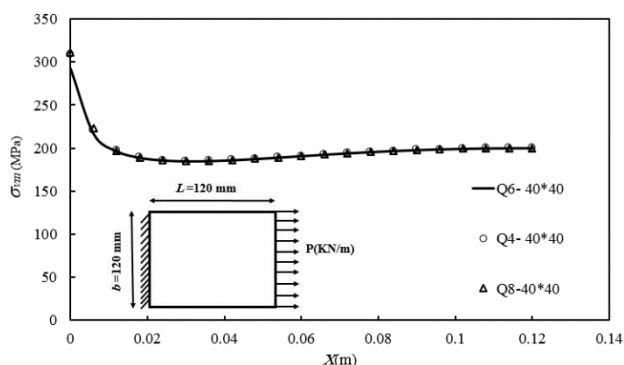
Fig. 8 Von-Mises stress through the plate length for Q4, Q6 and Q8 elements at y=120 \text{ mm} and 0 < x < 120 \text{ mm}
