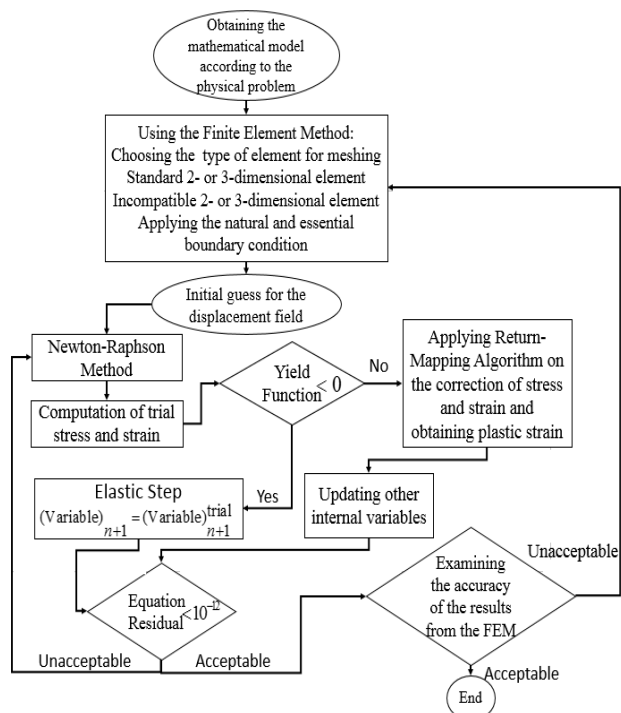
Fig. 4 Flowchart of numerical procedure
