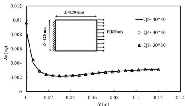
Fig. 9 Equivalent plastic strain through the plate length for Q4, Q6 and Q8 elements at y= 120\text{mm} and 0 < x < 120\text{ mm}
