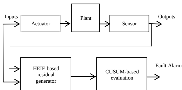
Fig. 4 Centralized fault detection block diagram
