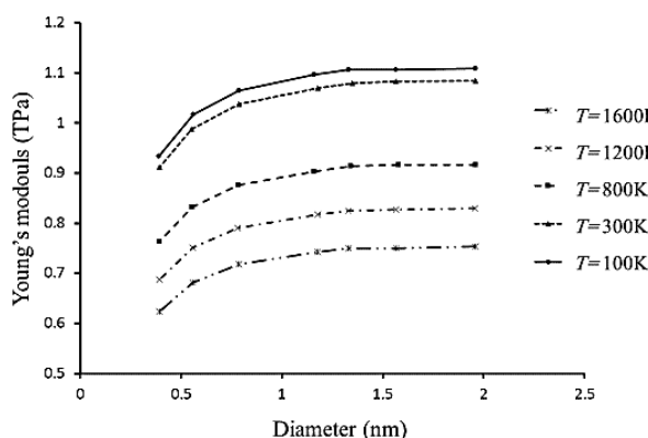
Fig. 6 Variations of Young's modulus in zigzag nanotubes with different diameters in different temperatures
