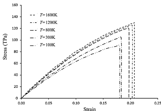
Fig. 11 Stress-Strain diagram in armchair nanotube with diameter of 0.8 nm in different temperatures
