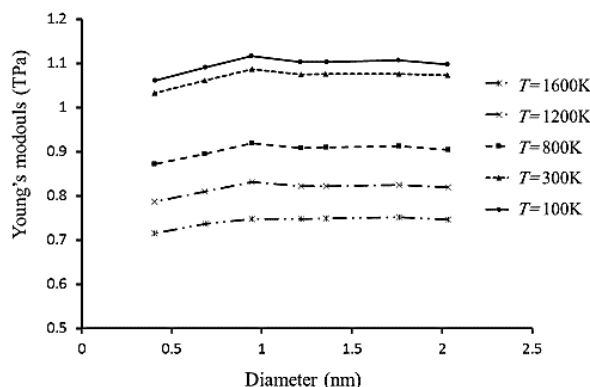
Fig. 7 Variations of Young's modulus in armchair nanotubes with different diameters in different temperatures
