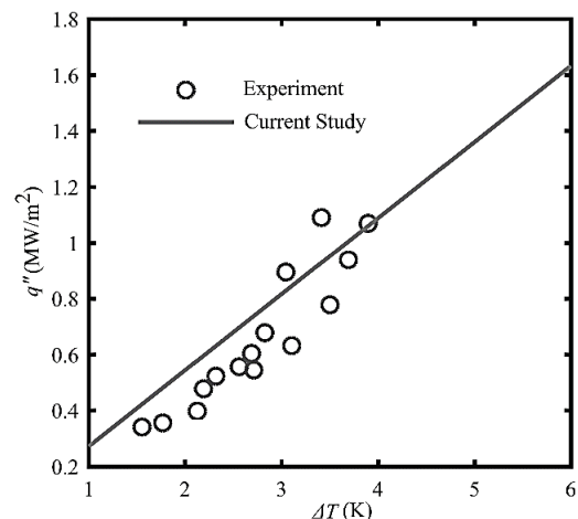
Fig. 3 Comparison of the variation of heat flux with respect to temperature difference of the current study with Wilmschurst and Rose experimental results [45]
