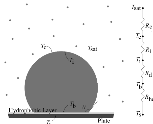
Fig. 1 Droplet state on plate and its thermal resistances
