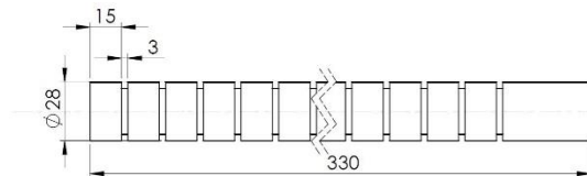
Fig. 1 The specimen of surface roughness test
