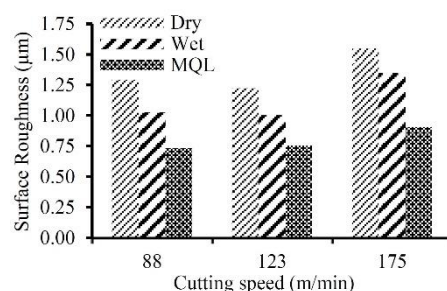
Fig. 5 Effect of cutting speed on surface roughness in dry, wet and MQL lubrication conditions
