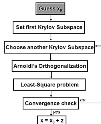
Fig. 1 GMRES Algorithm
