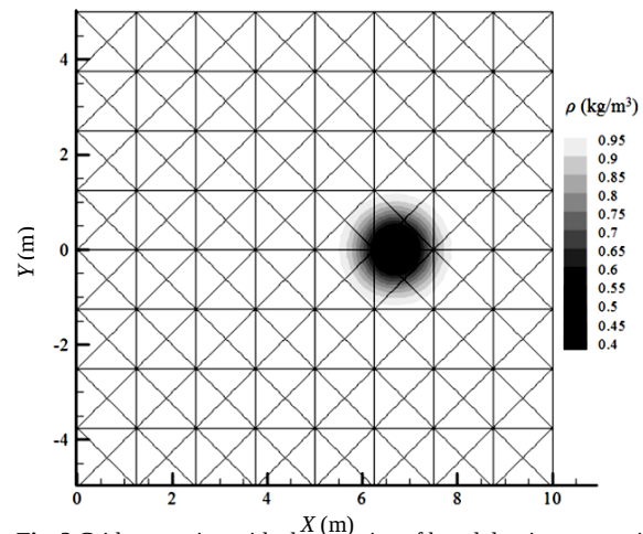
Fig. 2 Grid generation with element size of h and density contour in rotational isentropic flow
