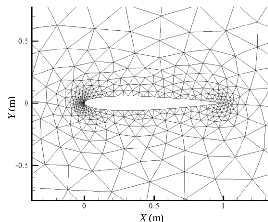
Fig. 8 Grid of transonic flow with 1298 elements
