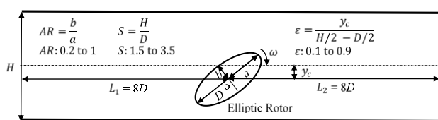
Fig. 1 The schematic of the problem geometry
