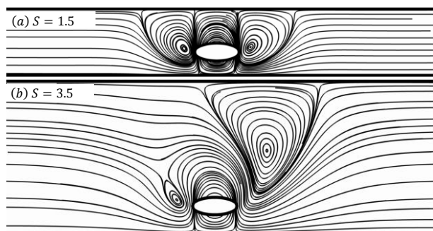
Fig. 13 Streamlines around the rotor with (a) S=1.5 (b) S=3.5 for AR=0.4 , \varepsilon=0.9 and t^*=1.5
