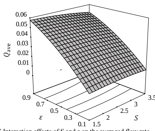
Fig. 16 Interaction effects of S and ε on the averaged flow rate
