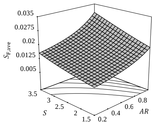
Fig. 18 Interaction effects of AR and S on the averaged entropy generation
