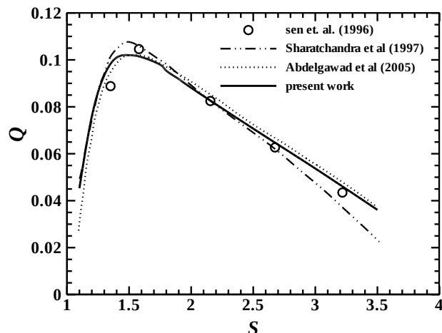
Fig. 5 Comparison of variations of Q vs. S parameter in the present study with those in literature for Re = 0.5 , \Delta P^* = 0.5 , \varepsilon = 0.9 and AR = 1
