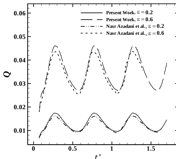
Fig. 6 Comparison of Q with dimensionless time ( t^* ) between the present study and Ref. [17] at Re = 1 , \Delta P^* = 0 and AR = 0.5 for two \varepsilon = 0.2 and 0.6
