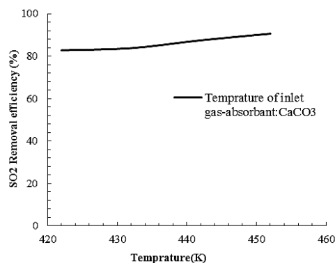
Fig. 24 The effect of temperature of inlet gas on efficiency of absorption– for \text{CaCO}_3 absorber
