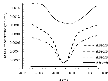
Fig. 22 The concentration of sulfur dioxide gas in different heights – for \text{NaHCO}_3 absorber
