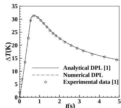
Fig. 4 The comparison of the DPL results with experimental data- 0.56 s pulse.
