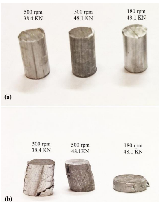
Fig. 8 The image of cutted samples a) before compression test b) after compression test
