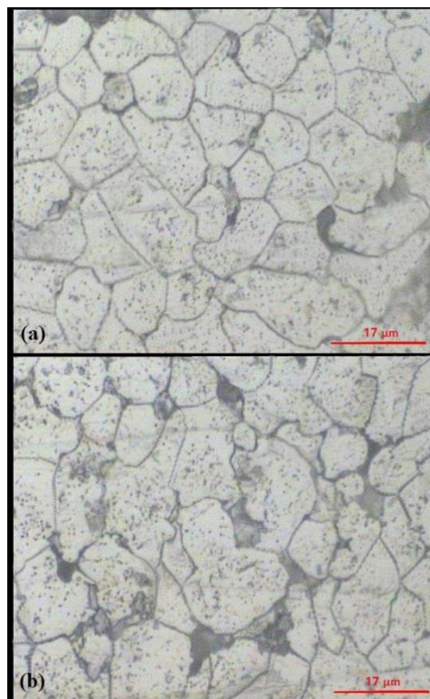
Fig. 5 a) Microstructure of extruded sample at rotational Speed and extrusion force of a) 500rpm, 48.1KN b) 500rpm, 38.4KN
