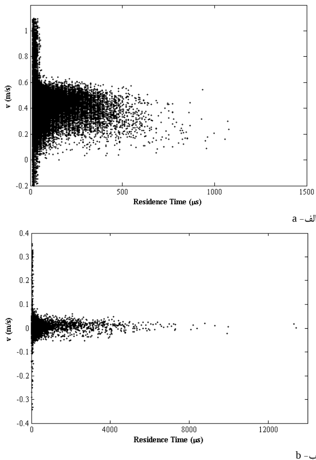
Fig. 5 velocity scattered diagram vs. residence time for two points in y/H=0.4 and a) x/e=0 , b) x/e=2
