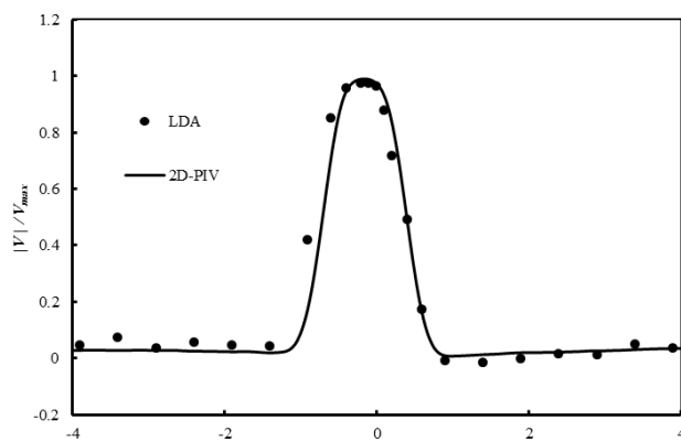
Fig. 7 comparison of measured mean velocity magnitude using 2D PIV [14] and LDA with RTW at y/H=0.17 ( Re=6000 )
