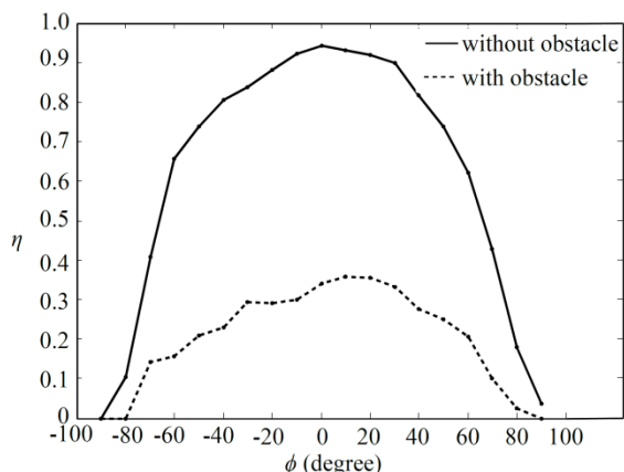
Fig. 5 The ratio of the practical workspace to the theoretical workspace ' \eta ' for different orientations of the 3-RRR parallel robot.
