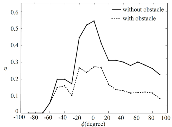
Fig. 8 The ratio of the practical workspace to the theoretical workspace ' \eta ' for different orientations of the 3-PRR parallel robot.
