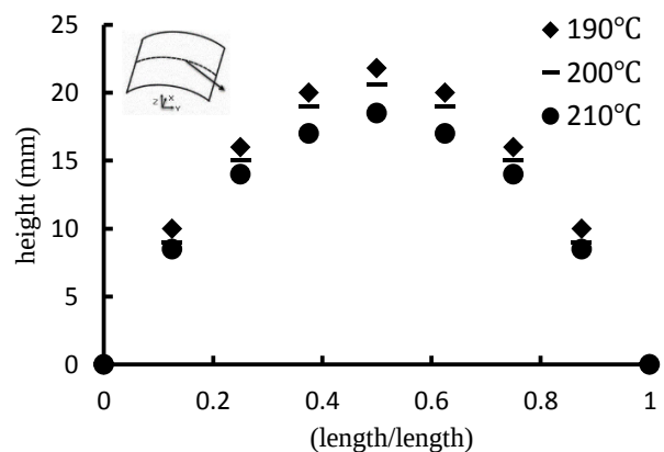
Fig.10 Effects of Mold's Temperature on Out of plane displacement at 20x20 Dimension (PVC/GF)
